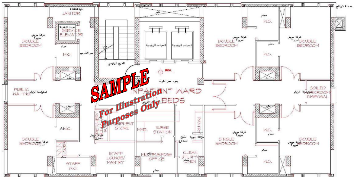
SECOND FLOOR
